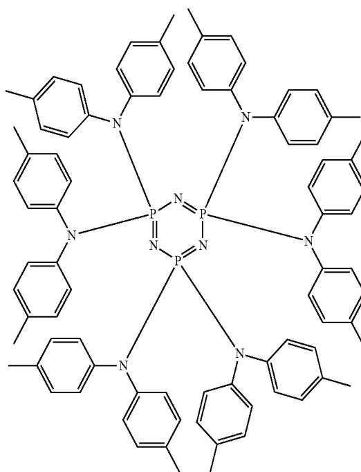
Compound 5
