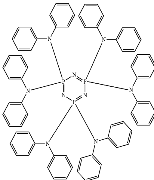
Compound 4
