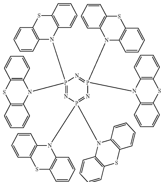
Compound 3
