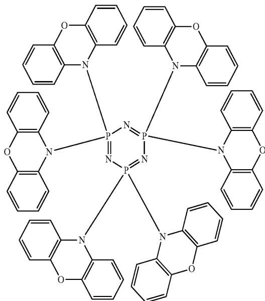
Compound 2
